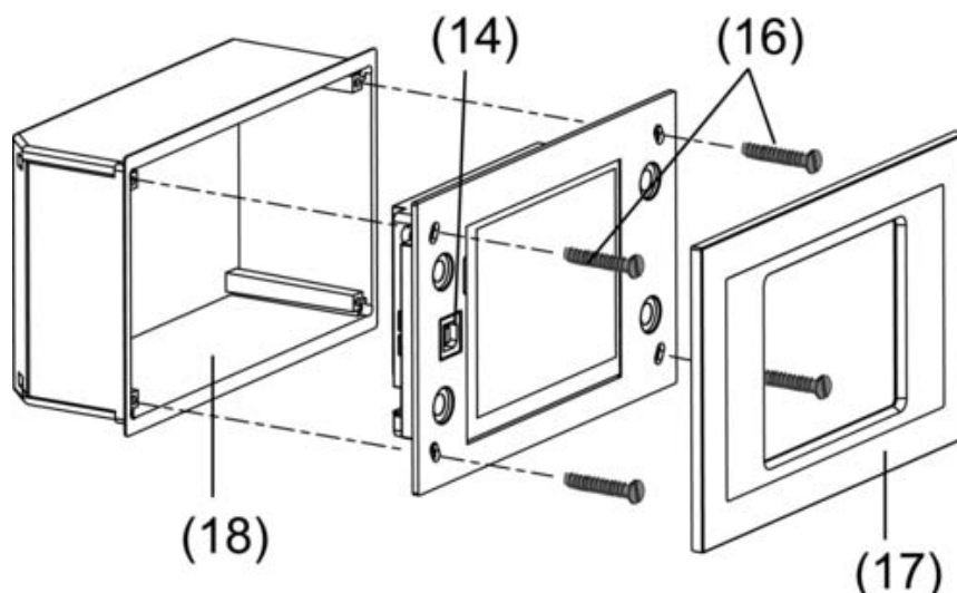
picture 5: Installation in panel-mounted housing.
